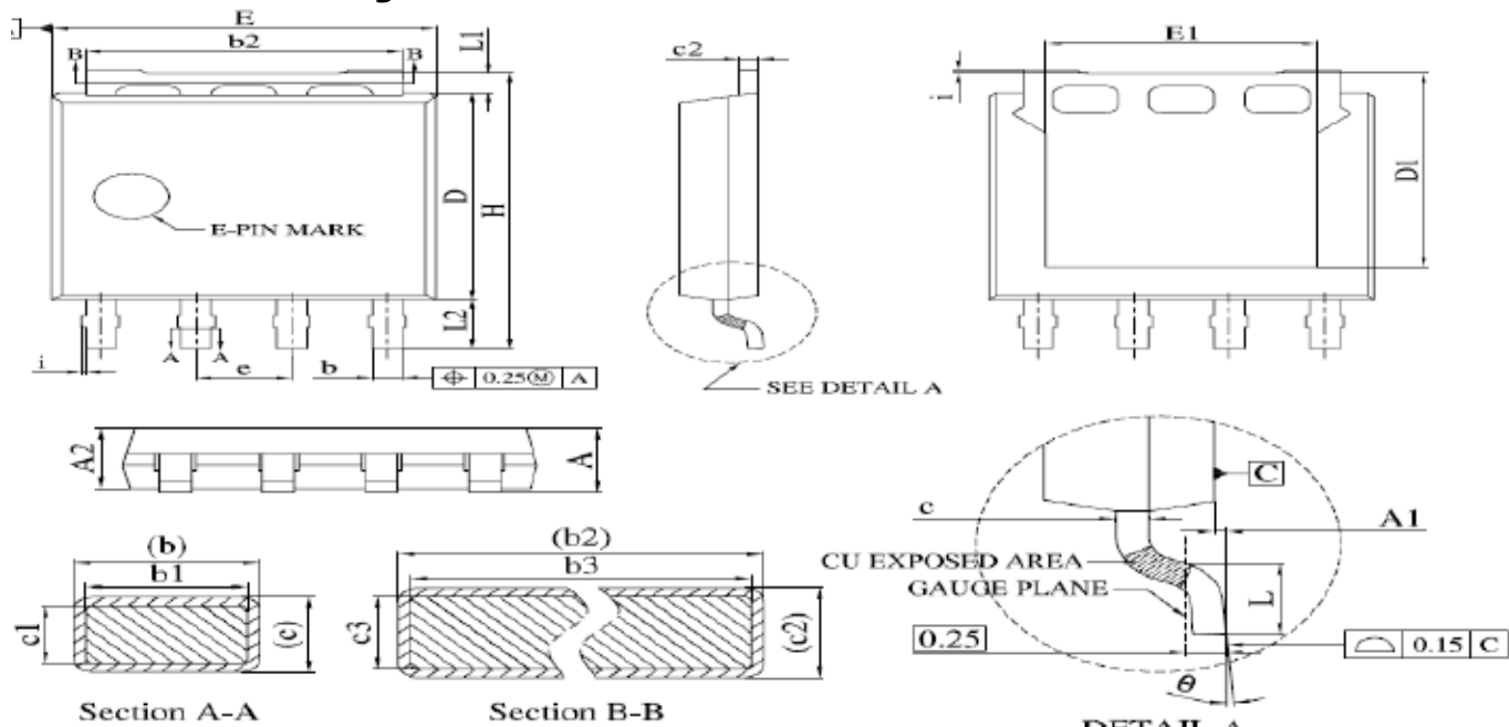
LFPAK5*6 Package
