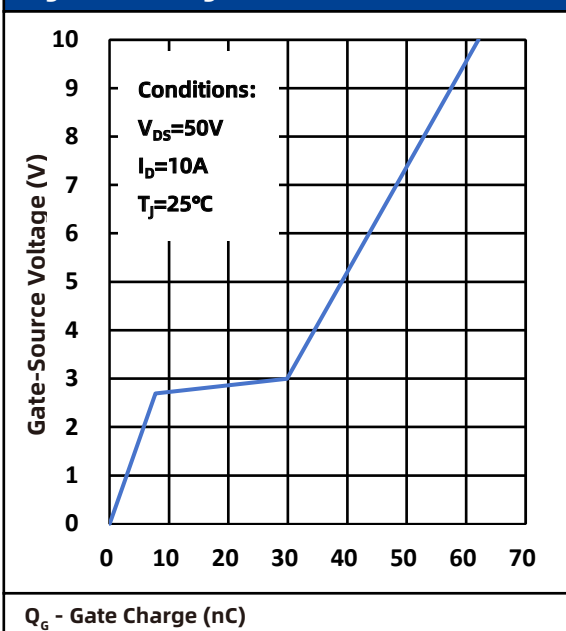
Fig.9 Gate Charge
