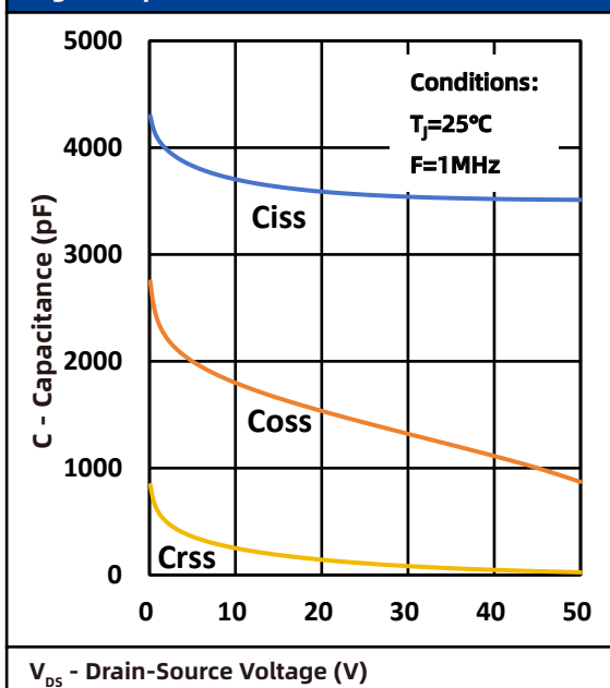
Fig.10 Capacitance
