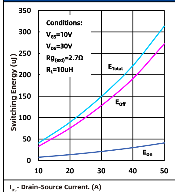
Fig.14 Switching Energy vs I DS
